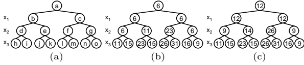
Figure 2: Search Trees for the Example
