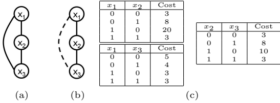
Figure 1: Example DCOP Problem
