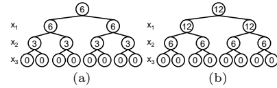
Figure 3: h -Values for the Example
