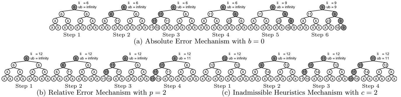
Figure 4: Execution Traces of ADOPT
