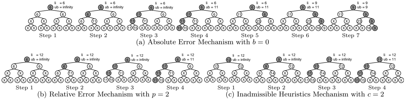
Figure 5: Execution Traces of BnB-ADOPT
