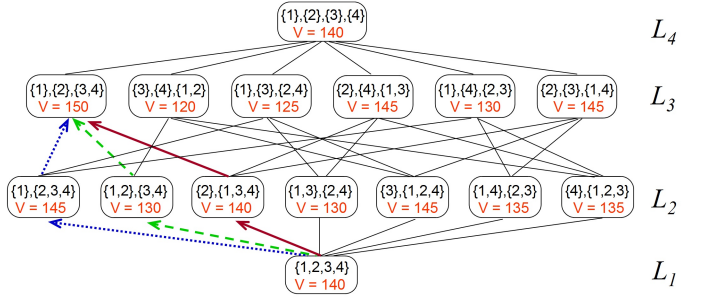
Figure 3: The coalition structure graph of 4 agents.
