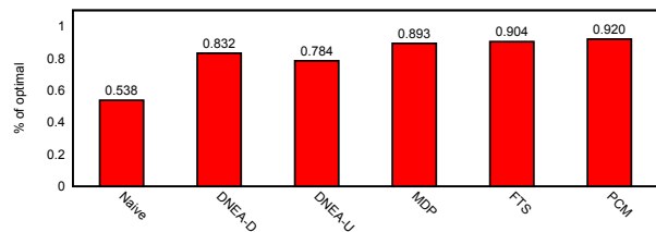
Figure 4: OptOP5PMix: Solution Quality as % of optimal (as determined by an offline solver).
