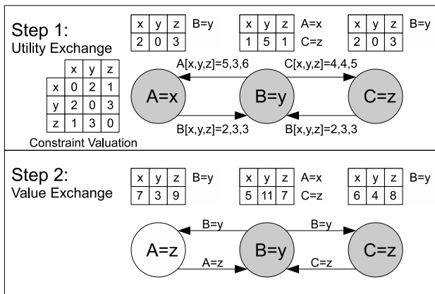
Figure 2: DNEA in action. Given constraint valuations shown at top and a random starting assignment of A=x , B=y , and C=z , DNEA finds the optimal assignment in one round of exchanges.
