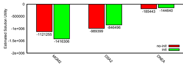
Figure 3: Estimated Solution Utility as a sum of DCOP utility for static scenario execution after 100 cycles, with and without an initial schedule. Closer to zero is better.
