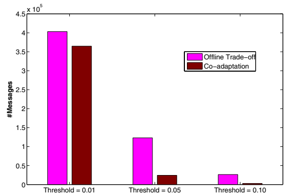
Figure 5: The performance of learned policies in the 20D network
