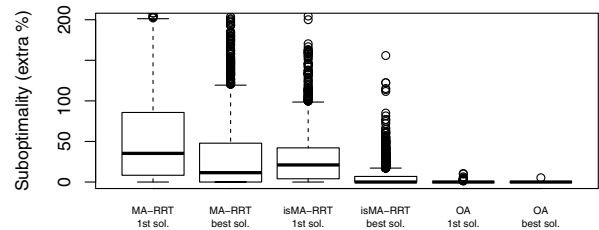
Figure 2: Solution quality
