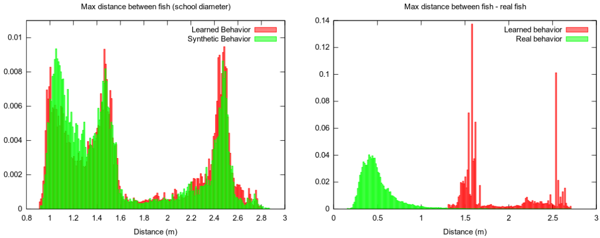
Figure 1: Learned behavior from synthetic and real data. Histograms of the learned behavior compared with the synthetic ( left ) and real ( right ) fish schools using one of the three schooling metrics: Maximum distance. The learned behavior matches the synthetic behavior very closely, but the same sensor model does not yield a close match on real fish.
