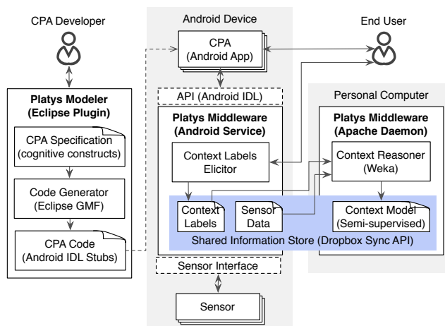
Figure 1: Platys framework includes a modeling tool and one or more middleware instances at run time.
