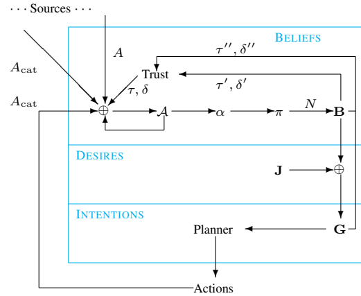
Figure 1: A schematic illustration of the BDI agent architecture within which the proposed model of trust is set.
