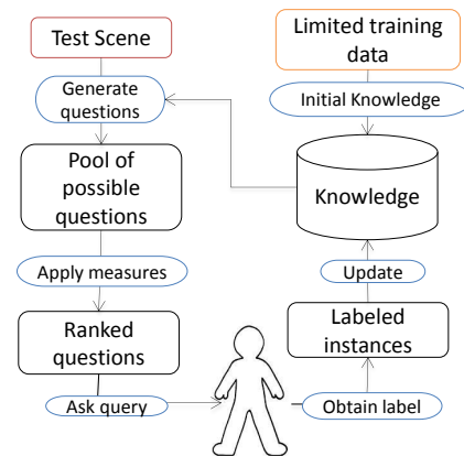
Figure 1: Proposed architecture.
