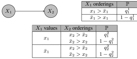
Figure 1: A PCP-net.
