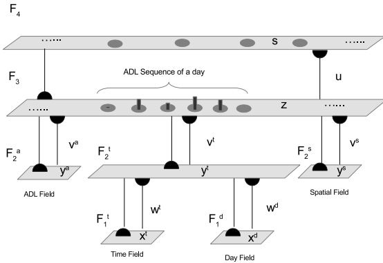
Figure 2: ST-ART model
