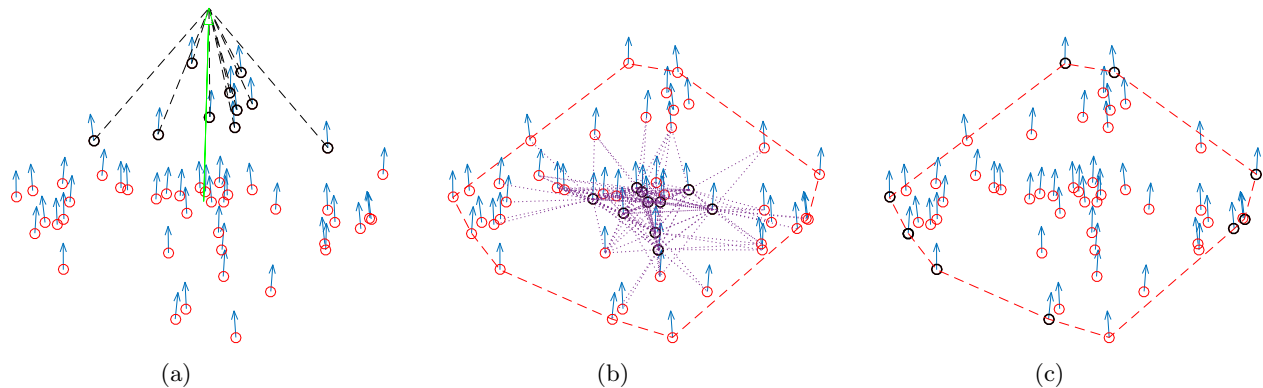
Figure 2: a) Front leaders are selected as the closest agents to a reference point which is generated at 1000 m away along the direction of the average heading angle of the swarm, b) Middle leaders are selected after removing agents from the convex hull, and those that have maximum connectivity with the remaining agents (purple dotted lines show neighbours of the leaders), and c) Periphery leaders are chosen from the convex hull. The number of leaders selected are about 20% leaders of the swarm and they are black in color. Leaders are selected at t = 0 .
