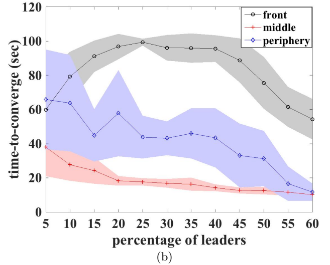
Figure 3: Variation of the time-to-converge with percentage of leaders for a) 50 agents and b) 100 agents. The lower bound denotes the time to converge for a single leader with no influence.
