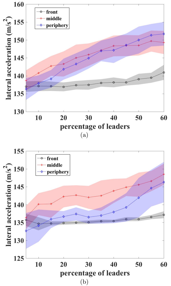
Figure 4: Variation of the lateral acceleration with percentage of leaders for a) 50 agents and b) 100 agents
