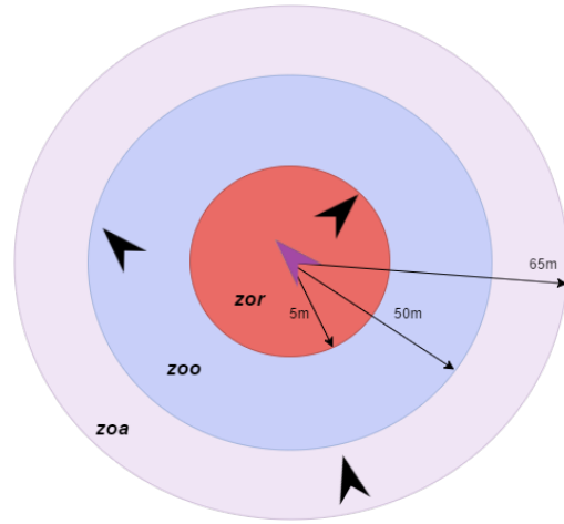
Figure 1: The zones of an agent – zone of repulsion ( zor ), zone of orientation ( zoo ), and zone of attraction ( zoa )
