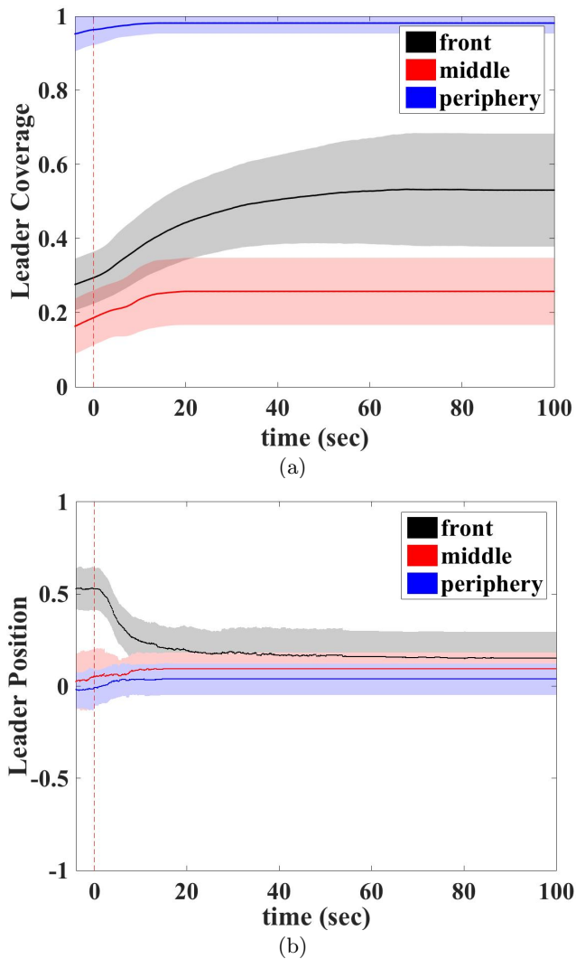
Figure 5: a) Leader coverage and b) Leader position for 50 agents and 15 leaders (30% leaders). The dotted vertical line represents the time at which we give the turn signal ( t = 0 ).
