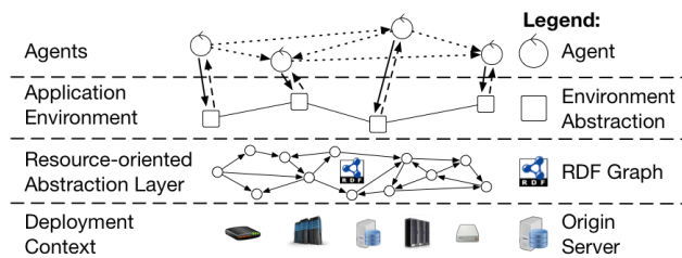
Figure 1: Layers of abstraction in hypermedia-driven agent environments.
