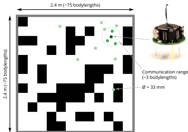
Figure 1: An example of Kilobots in a 2.4 \times 2.4 m ( 75 \times 75 bodylengths) arena. Kilobots can communicate to others within a radius of approximately 3 body lengths.
