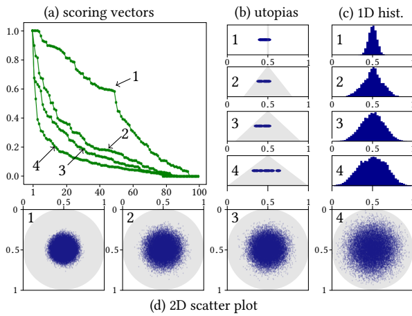
Figure 6: Results for weakly separable rules and utopic distributions (1) \mathcal{U}_{IE} , (2) \mathcal{U}_T^{0.2} , (3) \mathcal{U}_T^{0.1} , and (4) \mathcal{U}_T^0 .
