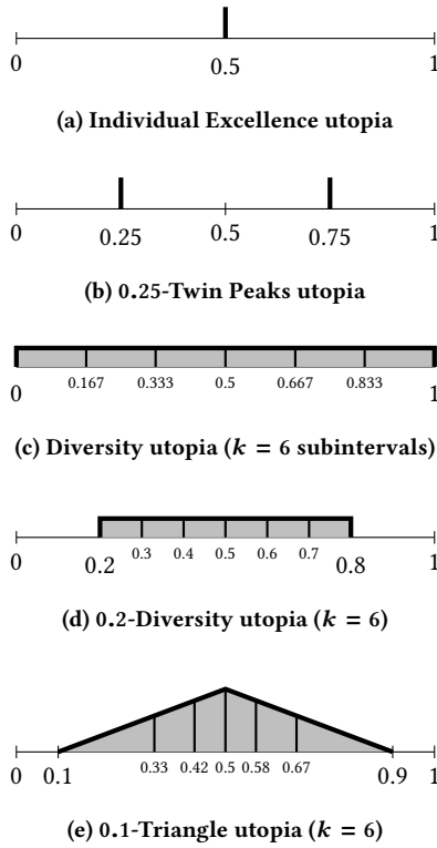
Figure 2: Several utopic distributions.
