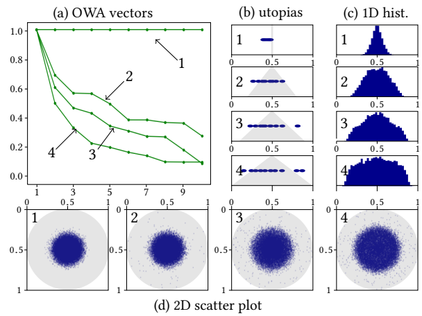
Figure 9: Results for OWA/Borda-based rules and utopic distributions (1) \mathcal{U}_{IE} , (2) \mathcal{U}_T^{0.2} , (3) \mathcal{U}_T^{0.1} , and (4) \mathcal{U}_T^0 .
