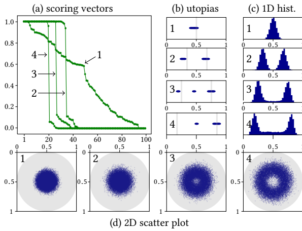
Figure 5: Results for weakly separable rules and utopic distributions (1) \mathcal{U}_{IE} , (2) \mathcal{U}_{TP}^{0.333} , (3) \mathcal{U}_{TP}^{0.25} , and (4) \mathcal{U}_{TP}^{0.167} .
