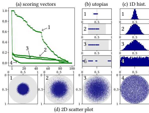
Figure 4: Results for weakly separable rules and utopic distributions (1) \mathcal{U}_{IE} , (2) \mathcal{U}_D^{0.2} , (3) \mathcal{U}_D^{0.1} , and (4) \mathcal{U}_D .
