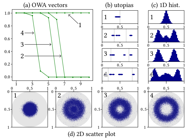
Figure 8: Results for OWA/Borda-based rules and utopic distributions (1) \mathcal{U}_{IE} , (2) \mathcal{U}_{TP}^{0.333} , (3) \mathcal{U}_{TP}^{0.25} , and (4) \mathcal{U}_{TP}^{0.167} .
