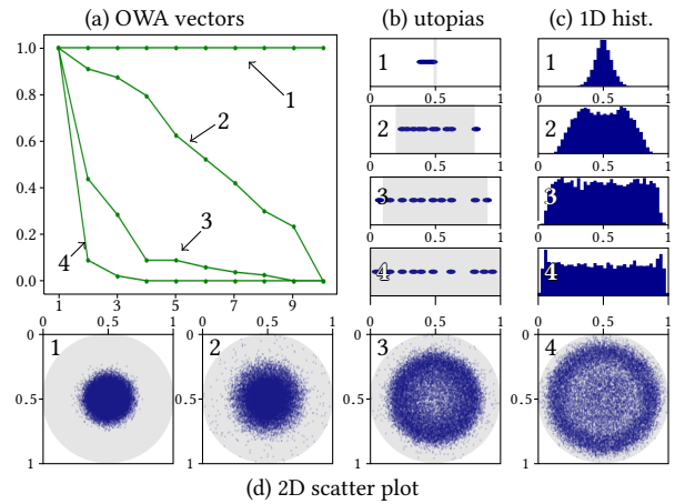
Figure 7: Results for OWA/Borda-based rules and utopic distributions (1) \mathcal{U}_{IE} , (2) \mathcal{U}_D^{0.2} , (3) \mathcal{U}_D^{0.1} , and (4) \mathcal{U}_D .
