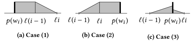
Figure 3: The cases for the cost of \text{EMD}(\mathcal{U}_D, d_W) . The cost associated with committee member w_i is the gray area.
