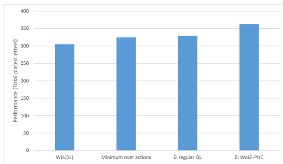
Figure 6: Performance of WLU(U) vs. different approximations of WLU(EI_{tot}) with different learning algorithms.
