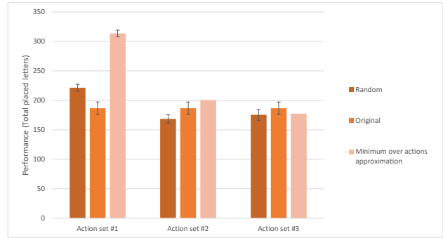
Figure 4: Performance of random choice vs. the original coordination method and the Minimum Over Actions WLU approximation.
