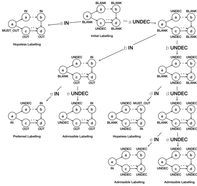
Figure 1: The behaviour of Algorithm 1 in calculating preferred extensions of a specific bipolar ABA framework. In the above, solid lines correspond to rules of the form \bar{\alpha} \leftarrow \beta and dotted lines to rules of the form \alpha \leftarrow \beta , where \alpha, \beta \in \mathcal{A} .
