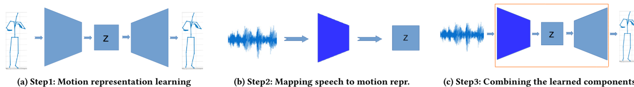
Figure 1: The proposed encoder-decoder DNN for speech-to-motion mapping.
