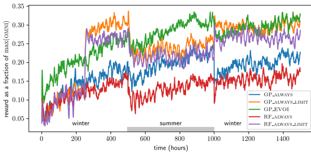
Figure 5: Reward accrued vs. time.
