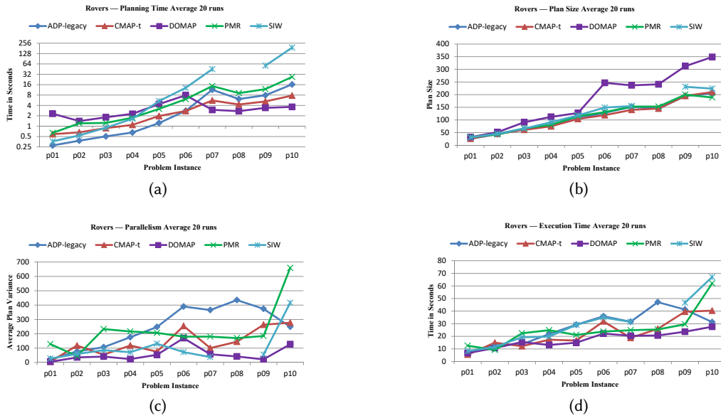
Figure 4: Results of experiments in the Rovers domain.
