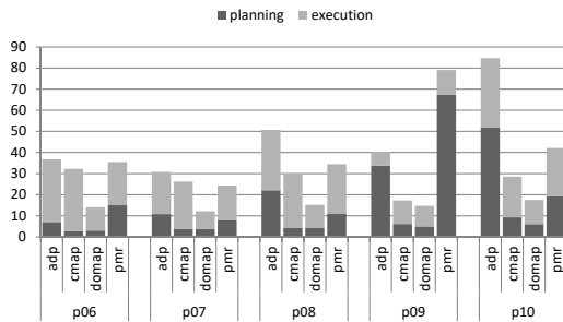
Figure 7: Planning and execution in the Floods domain.
