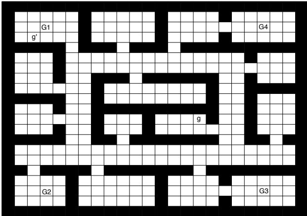
Figure 1: Source and target tasks in the map.
