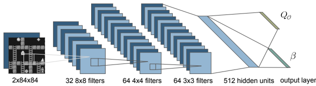
Figure 8: Neural Network Structure.
