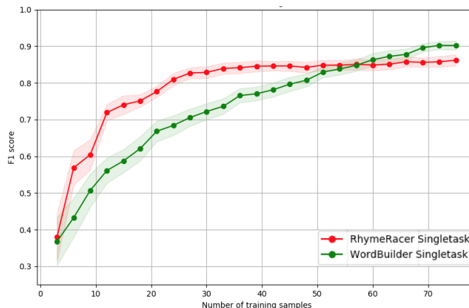
Figure 4: Learning curve for single-task models (F1-score). Both task models learn good classifiers with 60 samples
