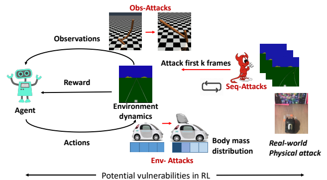
Figure 1: Analysis of adversarial attacks on DRL. RL environments are usually modeled as a Markov Decision Process (MDP), and its observation space, and environment (transition) dynamics may be attacked. We propose adversarial attacks that have improved computational efficiency by using the sequential nature of MDP, with attacks in both digital and physical environments.
