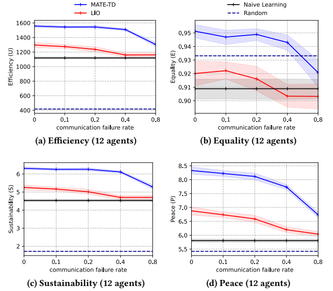
Figure 9: Performance of MATE, LIO, Naive Learning, and Random in Harvest after 5000 epochs w.r.t. different communication failure rates.
