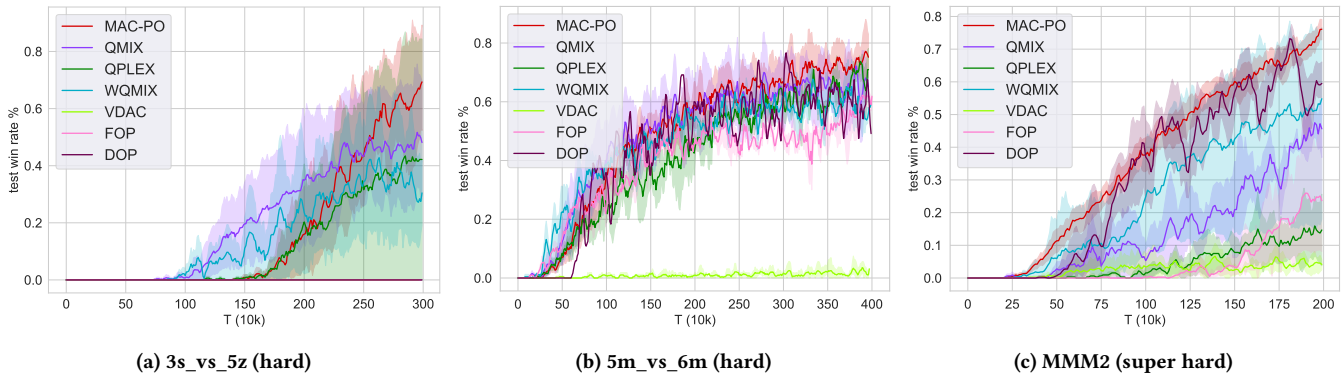
Figure 3: Comparison between MAC-PO and other MARL algorithms on three SMAC maps (from hard to super hard). MAC-PO achieves the best results with the optimal weighting scheme alone, outperforming the second best result by 11%, 4%, and 16% on each map, respectively.
