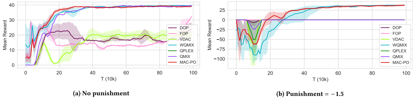
Figure 2: Average reward per episode on the Predator-Prey tasks for MAC-PO and other MARL algorithms of two settings, where MAC-PO shows the profoundly better convergence speed and pretty good results.
